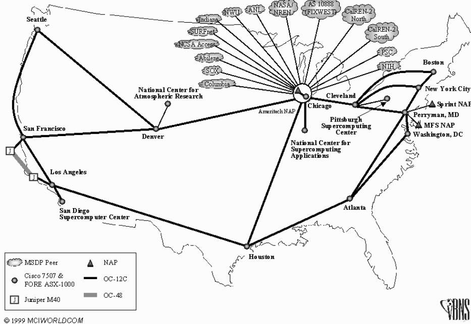
Figure 6: vBNS MBGP and MSDP peering topology.
